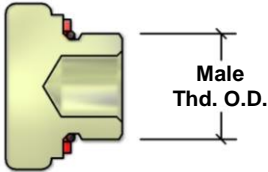
Male BSPP Port Connection (Washer / O-Ring)
