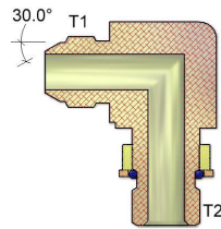
Male Komatsu To Bspp Male Adjustable 90° Elbow
