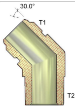
Jis Male To Bspt Male 45 degree Elbow
