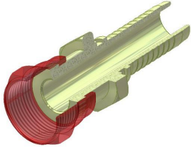
Straight Female Metric O-Ring Face Seal Fittings
