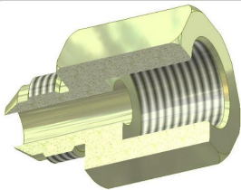
Male Jic X Metric Flat Face Adapters
