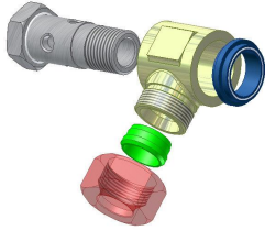
Adjustable Banjo Coupling Metric Thread With O-Ring Seal
