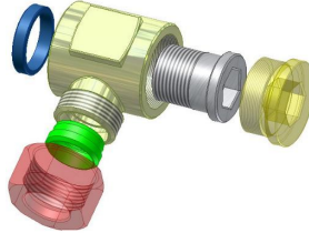
Full Passage Adjustable Banjo-Coupling BspP
