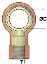
Metric Banjo To Female Npt
