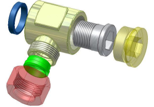
Full Passage Adjustable Banjo-Coupling Metric Thread
